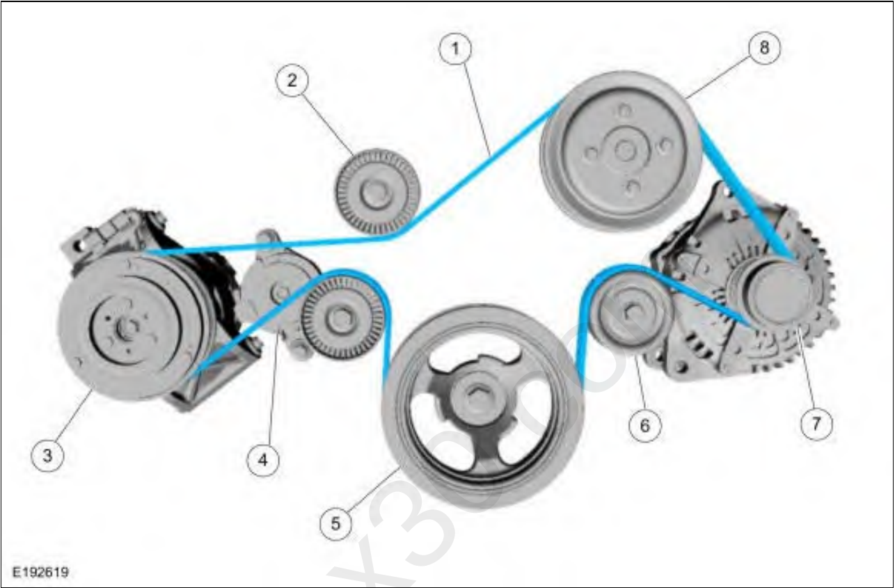
Fig 1: View Of Drive Belt And Pulley
